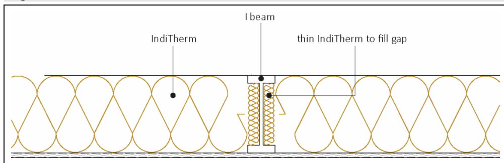
Figure 4 I beam section detail
