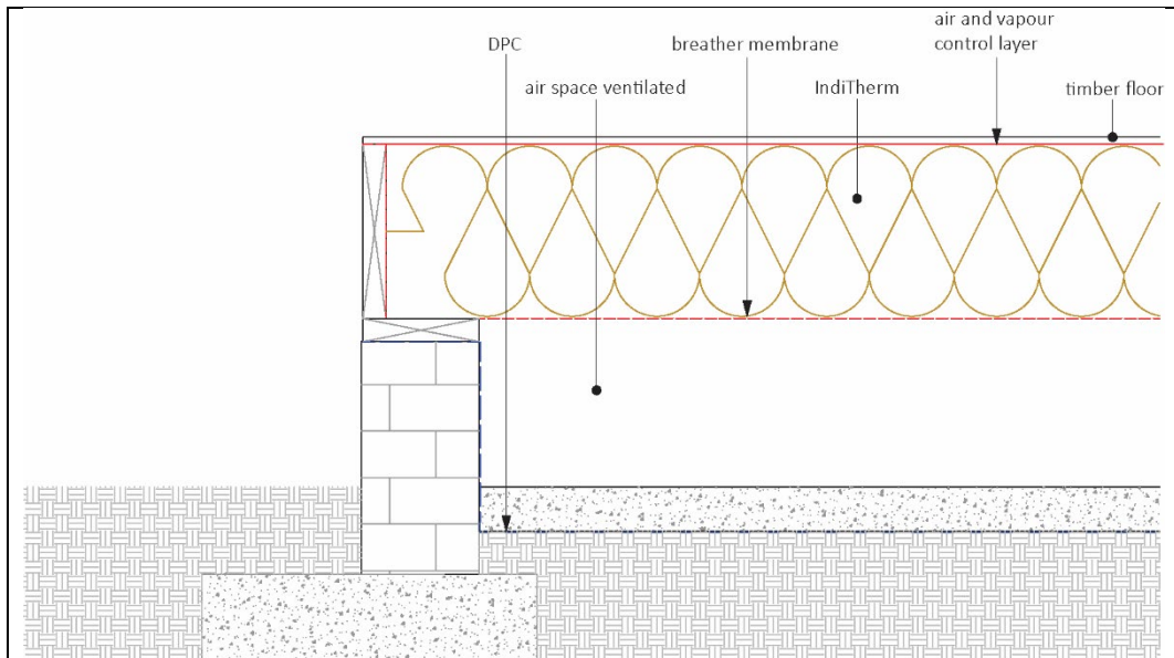
Figure 1 Typical suspended floor detail
